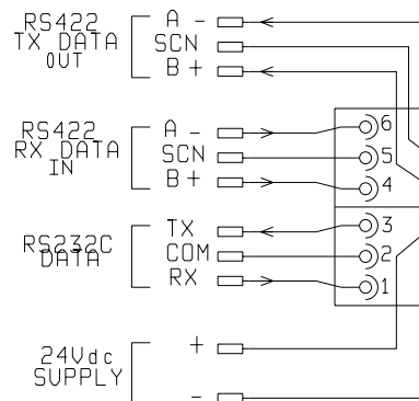
I.S. INTERFACE MODULE TYPE R007
